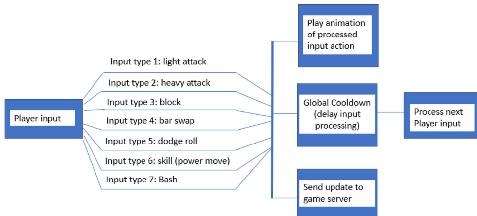
Figure 1: Elder Scrolls Online Player Input Processing.
