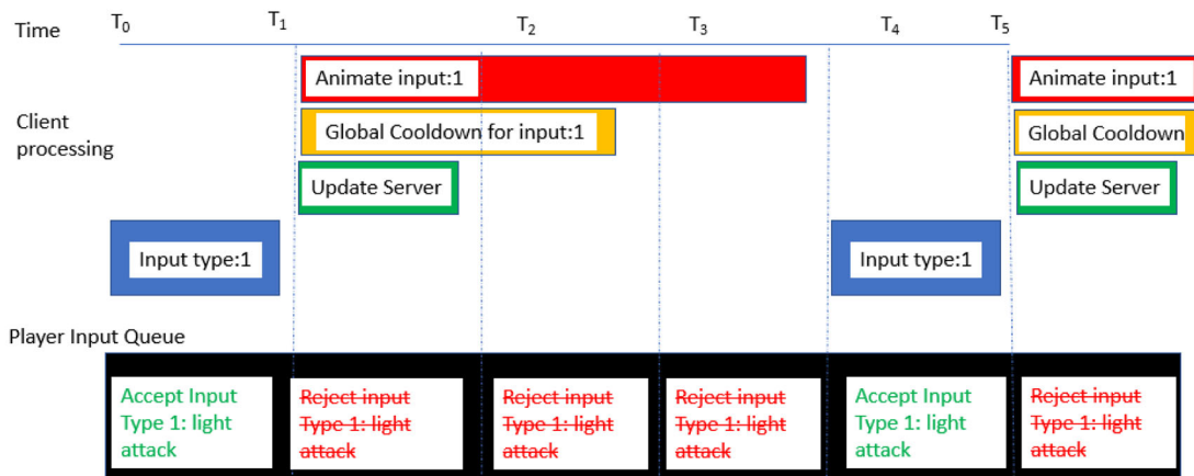
Figure 2: Elder Scrolls Online Intended Input Throttling Behavior.
