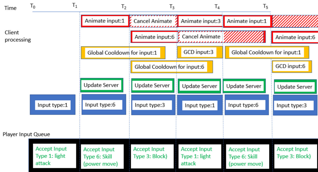
Figure 3: Elder Scrolls Online Unintended Throttling Behavior.
